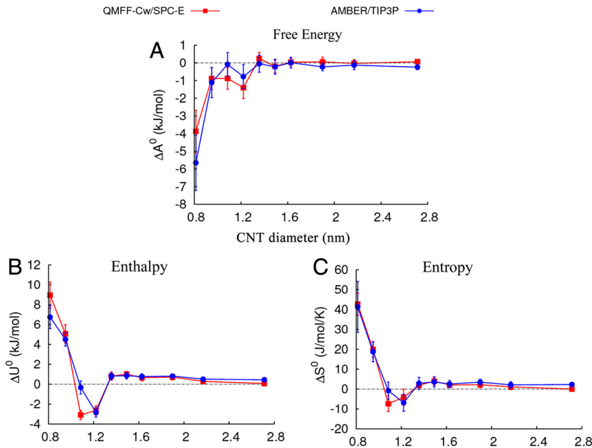
Fig. S5. Comparison of the (A) free energy \Delta A^0 , (B) enthalpy \Delta U^0 , and (C) entropy \Delta S^0 of water confined in 10 carbon nanotubes (CNTs) with the simple point charge-extended (SPC-E) water model (this study, red squares) and with the unoptimized parameters of the AMBER96 force field for carbon and the TIP3P water model (oxygen-carbon parameters of \epsilon_{C-O} = 0.392 kJ/mol and \sigma_{C-O} = 3.275 Å, blue filled circles) (1). The good agreement indicates that the results presented in this study are fairly insensitive to the choice of interaction potentials. As a figure of merit, we calculate the free energy of water inside the 0.8-nm (6,6) CNT to be -3.98 kJ/mol using the two-phase thermodynamics method, which is in good agreement with the value of -3.34 kJ/mol in ref. 1 from potential of mean force calculations.
