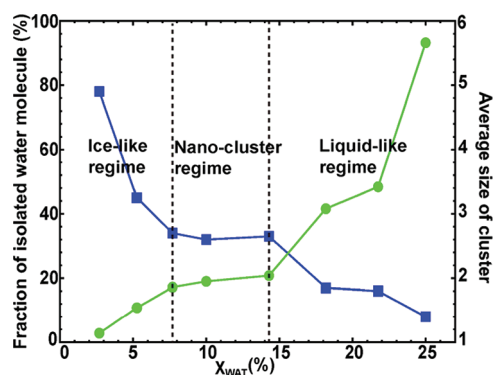
Figure 2. Fraction of isolated water molecule (blue) and the average cluster size (green) as a function of water content ( \chi_{\text{WAT}} ). The number of waters in each cluster increases with increasing of \chi_{\text{WAT}} . From previous IR experimental study, 12 the water molecule in the similar IL system (BMIm + /TFSI - ) with \sim 7 mol % shows IR peak splitting of symmetric and antisymmetric stretching modes, inferring that the water in this water content regime is isolated and very different from liquid phase water. This compares with our simulation results.
